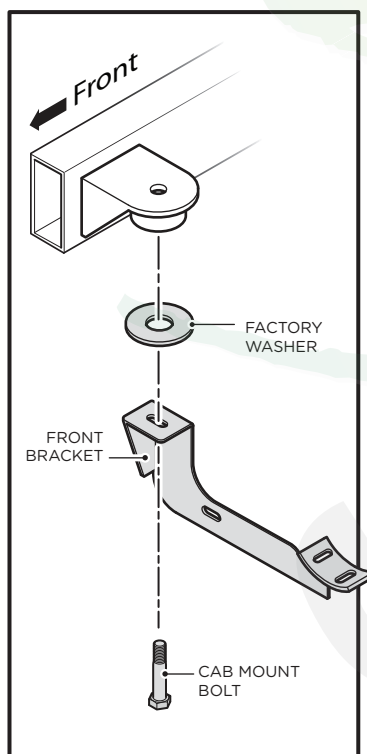
Front Bracket
