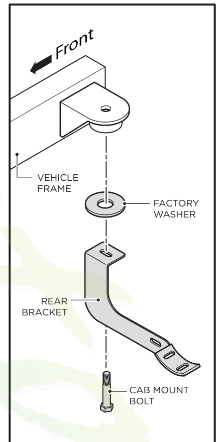
Rear Bracket
