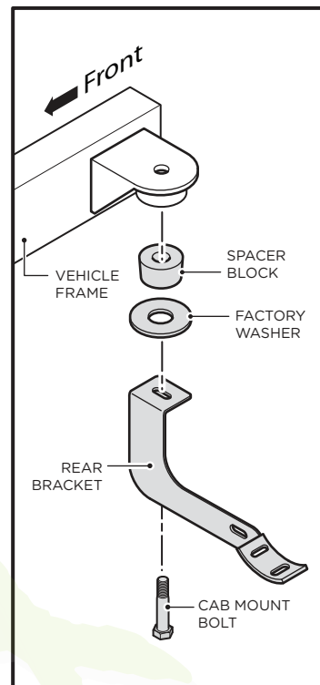
Rear Bracket
