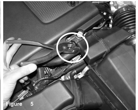
Figure 5 Depress the wire tension clamp on the crank case breather hose and pull it away from the crank case vent box.
