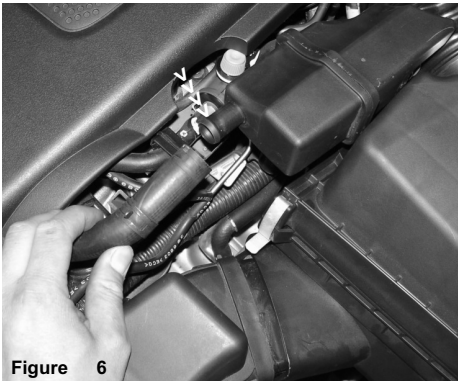
Figure 6 Once the tension clamp is pulled away, continue to pull the hose away from the CCV box.
