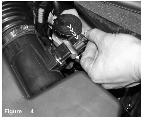
Figure 4 Press the clip on the harness connector and pull the electrical harness from the mass air flow sensor.
