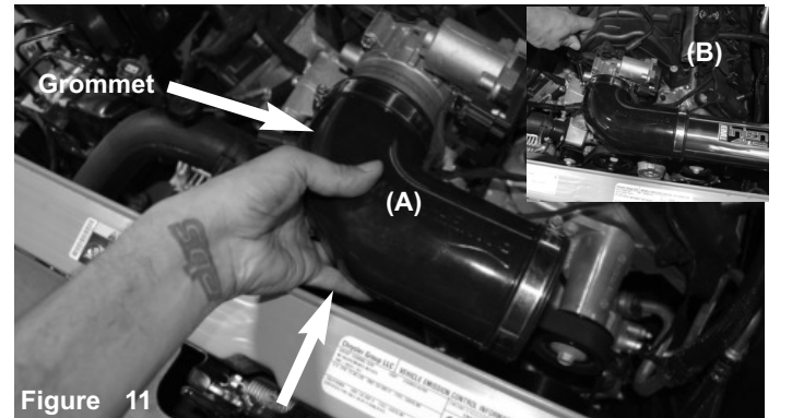
Install the elbow with clamps provided to the throttle body. Make sure the short side with grommet is on the throttle body. (B)
